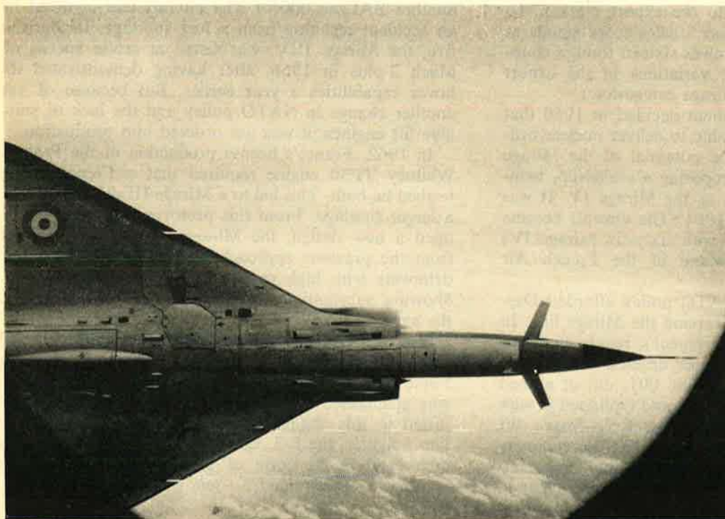
Equipped with a canard for improved low-speed aerodynamic characteristics, the Milan will have excellent STOL capability. The Milan is about to enter intensive flight testing.
