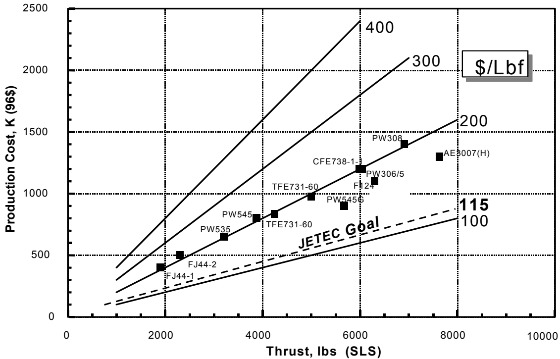
FIGURE A-2: JETEC COST GOAL IN COMPARISON TO EXISTING SYSTEMS. CLEARLY, INNOVATIVE, LOW-COST DESIGN AND MANUFACTURING TECHNIQUES MUST BE DEVELOPED TO MEET THIS GOAL.
