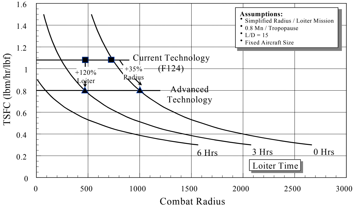
FIGURE A-1: THE PERFORMANCE PAYOFF OF A NOTIONAL COMBAT UAV UTILIZING TECHNOLOGIES FROM THE SUCCESSFUL DEMONSTRATION THE JETEC PHASE III GOALS.
