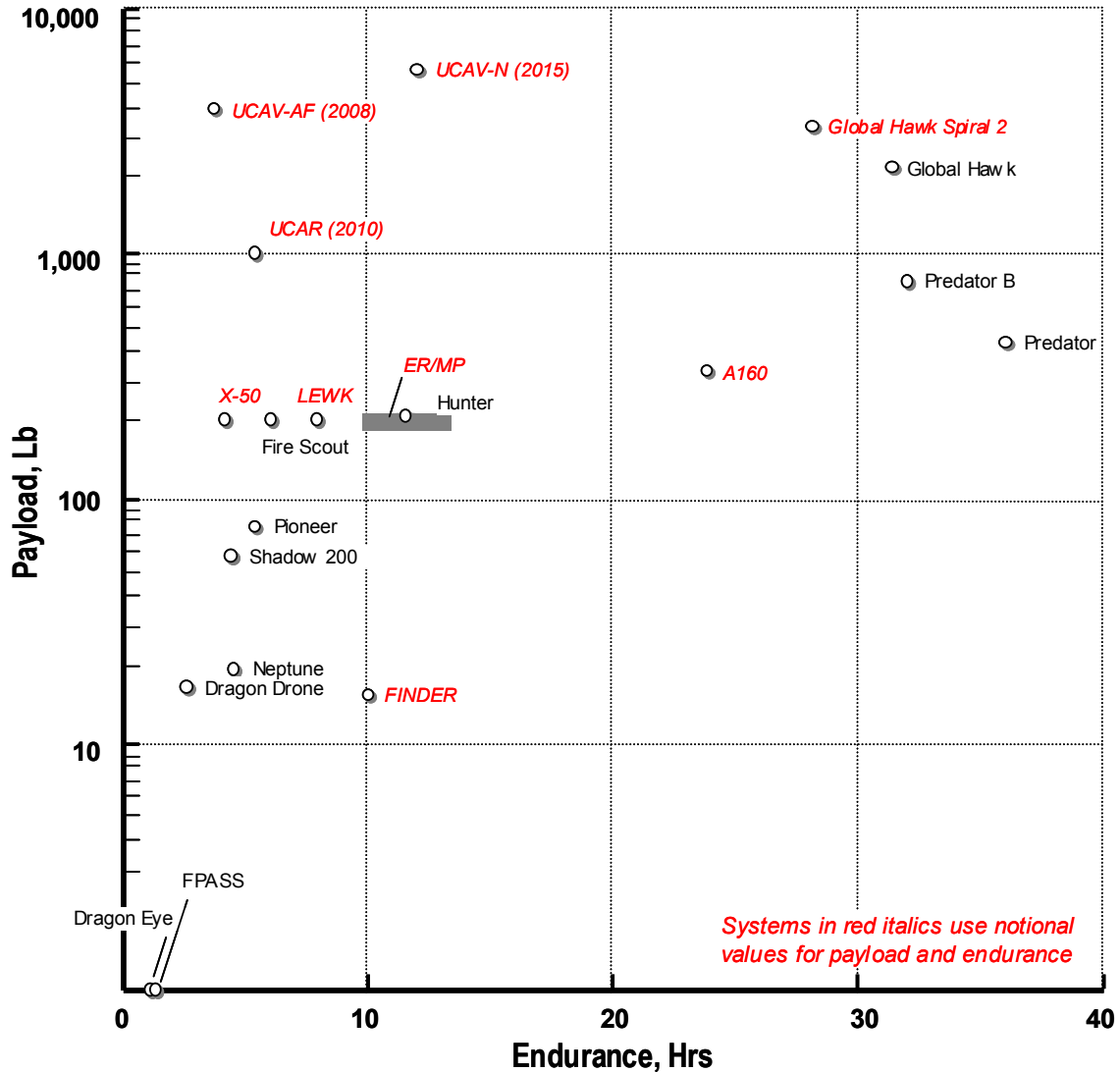
FIGURE 4.2-1: UAV PAYLOAD WEIGHT VS. ENDURANCE.
