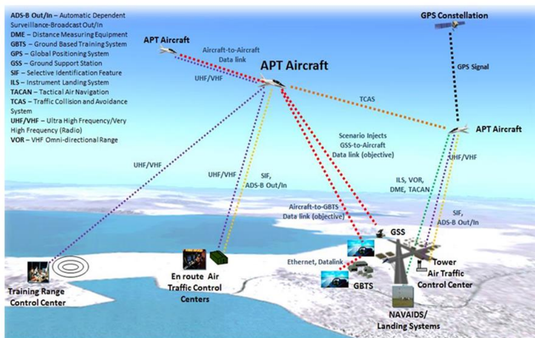
Figure 6. APT T-X Operational View
